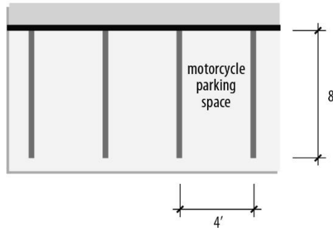
Figure 10-2: Motorcycle Parking Space Dimensions
