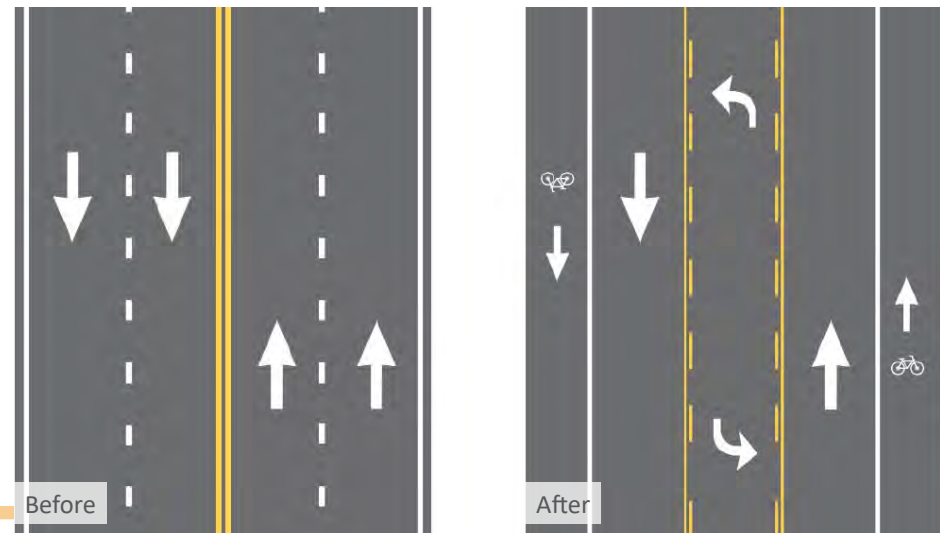
FIGURE 16. ROADWAY RECONFIGURATION
